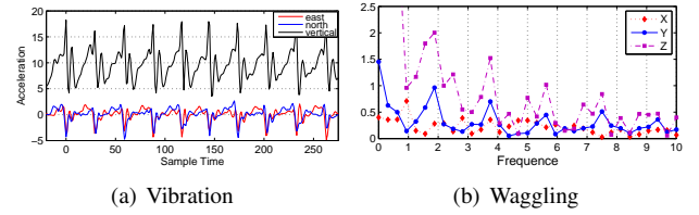
Fig. 2. a) the raw data of acceleration of a walking user; b) the FFT of accelerations along the walking orientation (Y), perpendicular (X) and to the sky (Z).
