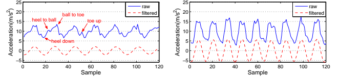
(a) The raw vertical acceleration and filtered vertical acceleration while user is walking at a normal pace. (b) The raw vertical acceleration and filtered vertical acceleration while user is walking at a fast pace.
