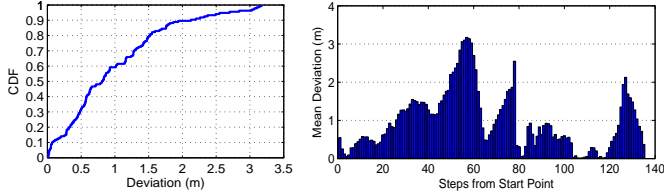
Fig. 9. Single users's tracking result by movement vectors.
